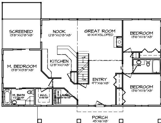
FIRST FLOOR PLAN A-4
